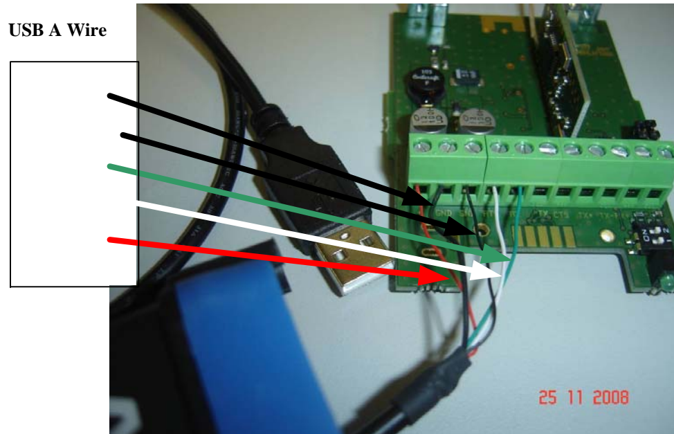
USB A Male connected to an ARF USB Modem
